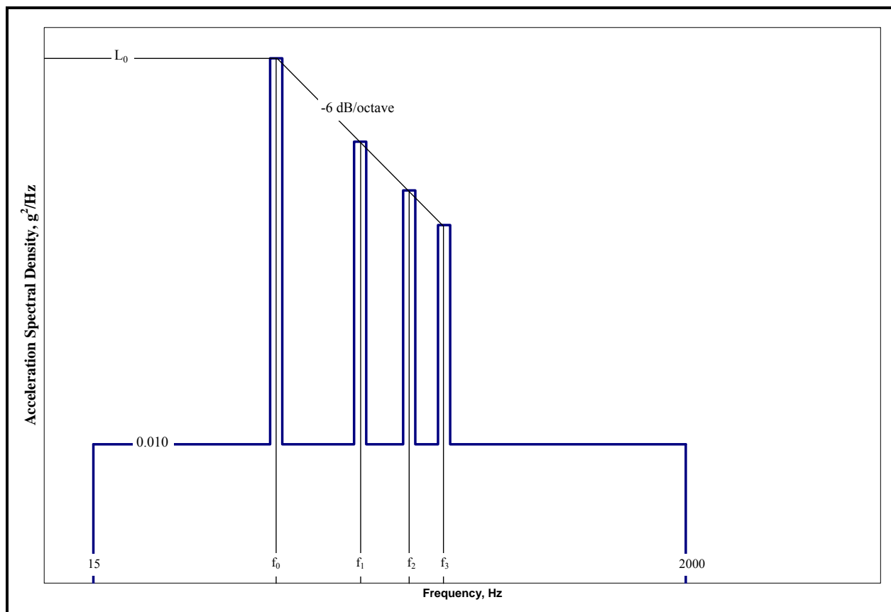
Figure 514.6D-2 – Category 13 - Propeller aircraft vibration exposure. (Same as Annex C, Figure 514.6C-7.)
