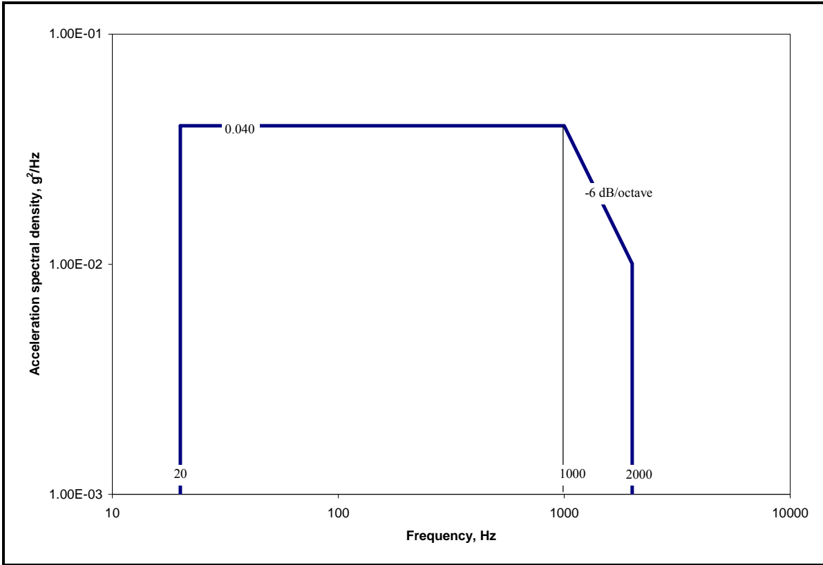
Figure 514.6E-1. Category 24 - General minimum integrity exposure. (Test duration: One hour per axis; rms = 7.7 gs)
