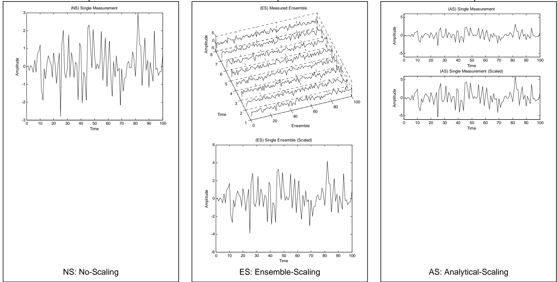
Figure 525-1. Basic TWR test modes as related to time trace scaling.
