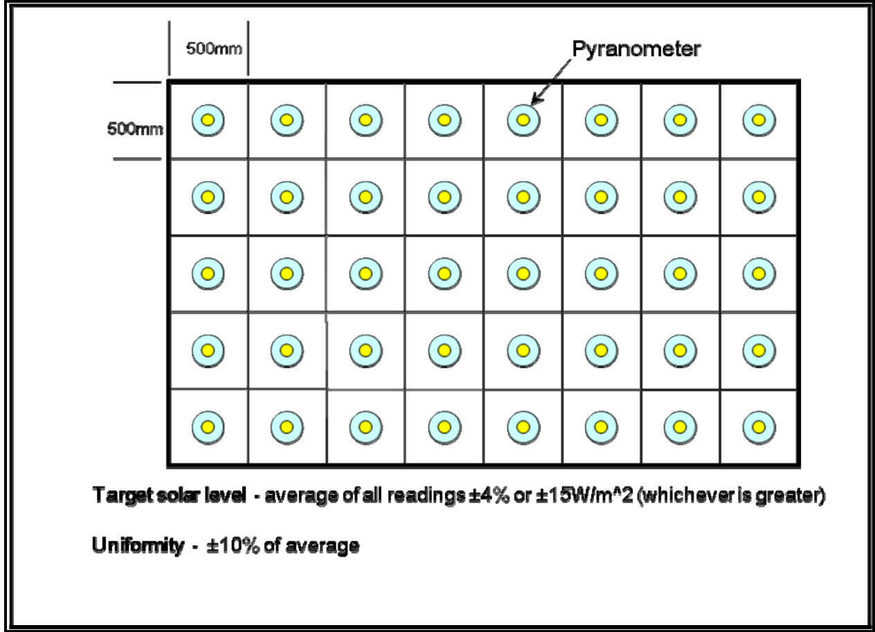
Figure 505.5C-1. Example of establishing target and uniformity levels over surface target plane.
