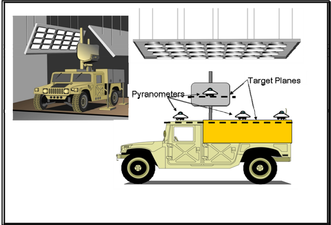
Figure 505.5C-4. Example 3 – Multiple solar surface target planes.
