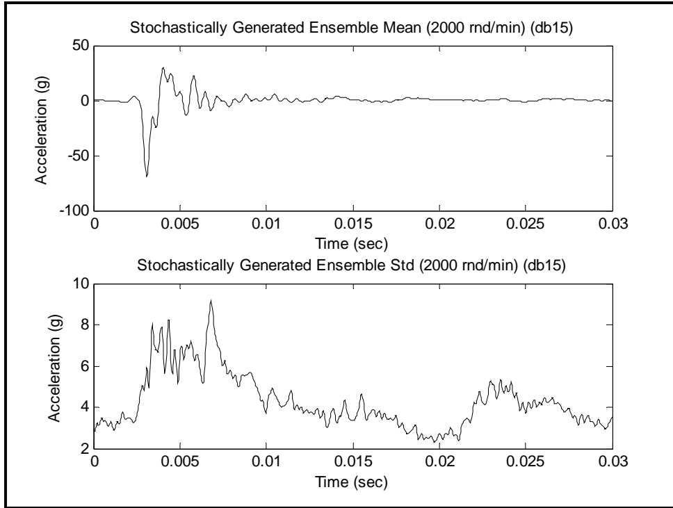
Figure 519.6B-8c. Ensemble and stochastically generated pulse ensemble random component standard deviation (2000 rnd/min).
