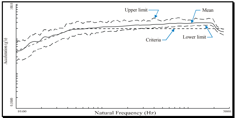
Figure 516.6C-3b. SRS comparison for functional test for flight materiel.
