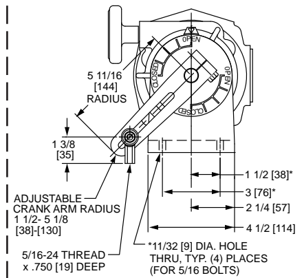
Mounting Option D
