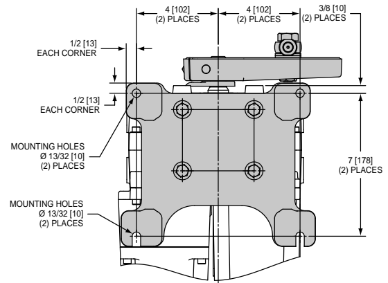
WITH OPTIONAL MOUNTING PLATE
