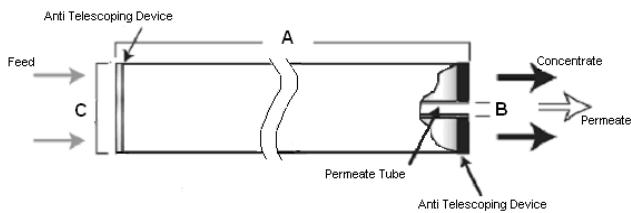
Figure 1a: Element Dimensions Diagram (Female) – 4040 & 8040
