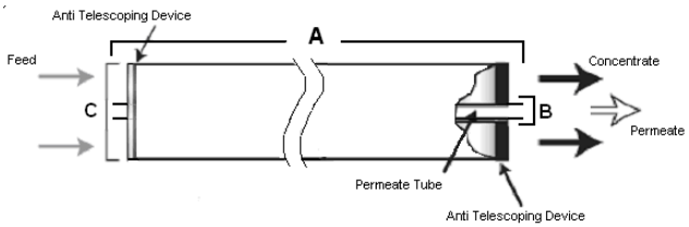
Figure 1b: Element Dimensions Diagram (Male) - 2540
