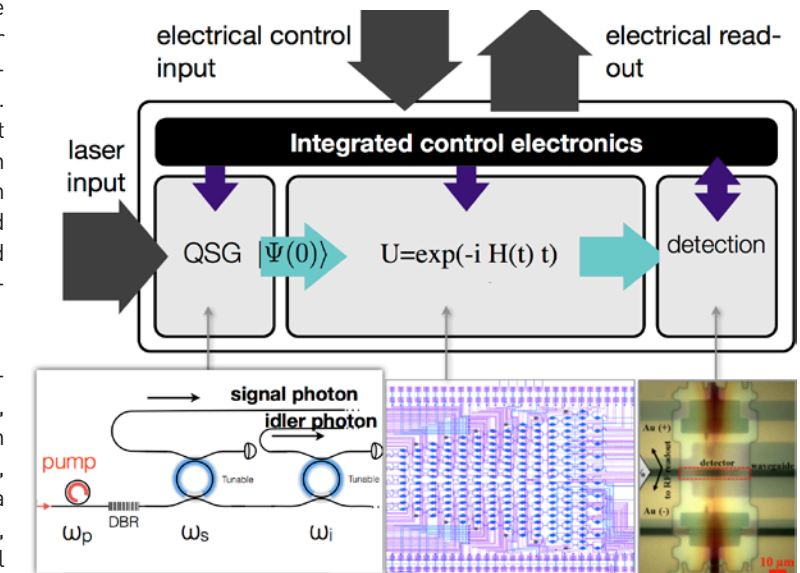
Figure 1. Process flow: A user-provided algorithm is converted to a machine executable using a compiler for the classical central processing unit (CPU) and the quantum photonic processor (QPP). The classical processor executes 'experiments' on the QPP for a specified number of repetitions or until an output with sufficient certainty is produced. The QPP consists of quantum state generator (QSG), the quantum photonic unitary (QPU), and the SNSPD detector array. Bottom row: Examples of QSG, QPU, and waveguide-integrated SNSPD (with the Karl Berggren group at MIT).
