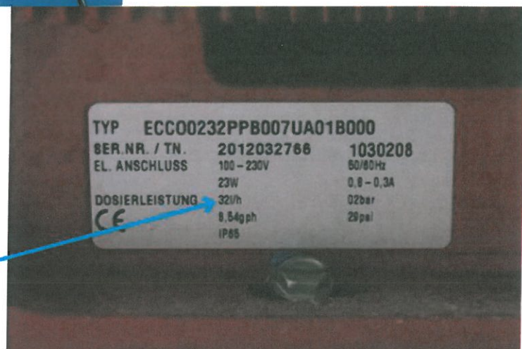
Close up of the name plate of an individual feed pump. Dosierleistung is translated as dosing capacity or maximum flow.
