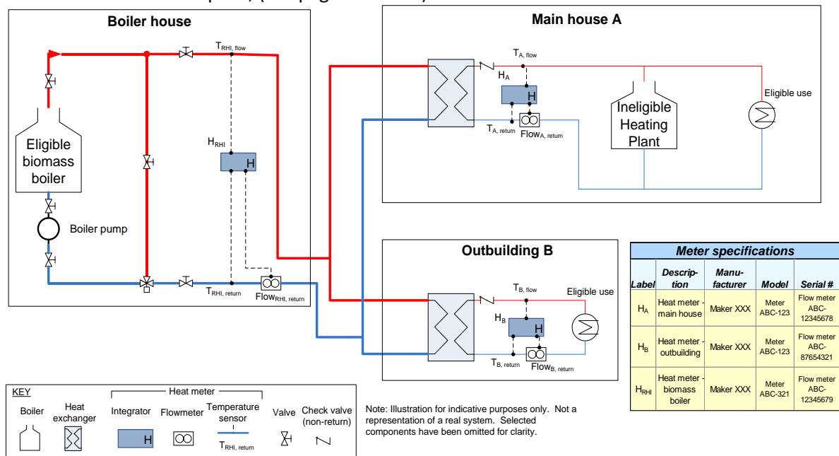
Figure One: Illustration of possible metering arrangement for a complex installation where decentralised ineligible plants (in this example, fossil fuel boilers) are located
