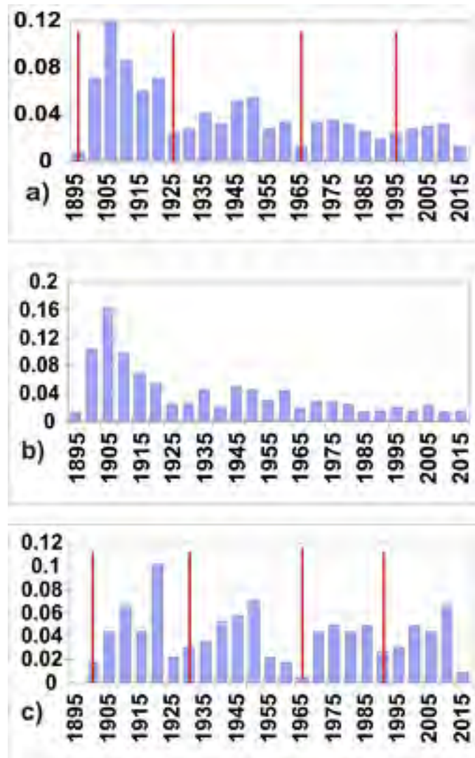
Figure 10. The distributions of the relative number of the EQ with M \geq 7.5 per five-year interval: a) - for the whole Earth, b) - for the Northern Hemisphere and c) - for the Southern Hemisphere. The labels on the horizontal axes correspond to upper limit of each five-year interval
