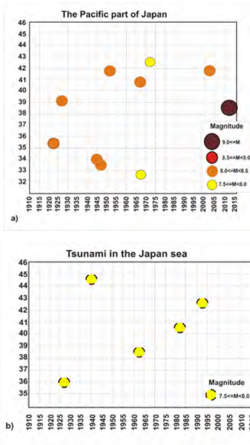
Figure 15. The two-dimensional distributions of the TEQ (per latitudes and five-year interval): a) - in the Pacific part of Japan, b) in the Sea of Japan. The vertical axes are the latitudes of the TEQ epicenter. The labels on the horizontal axes correspond to the upper limit of each five-year interval. The magnitude legend is in bottom-right corner of each plot.
