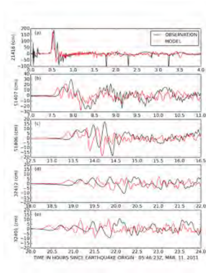
Figure 2. Comparison of RIFT model result without depth-correction with observations at DARTs for the Mar. 11, 2011 Tohoku Tsunami. The model is forced with the USGS finite fault solution ( M_w=9.0 ). See Section 3.3 for details of forcing parameters used.
