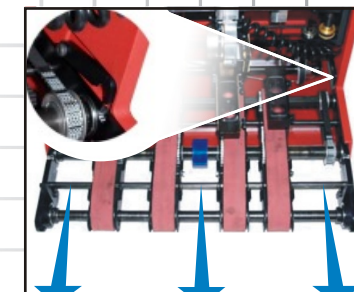
Belt Carriage
