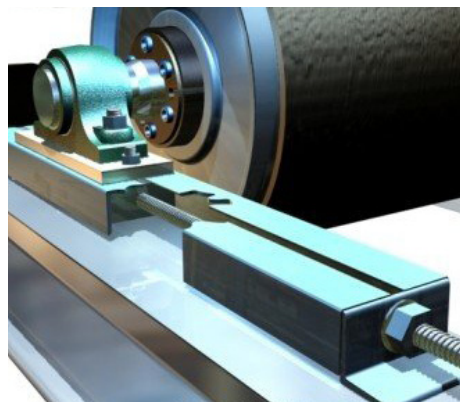
Screw Take Up
