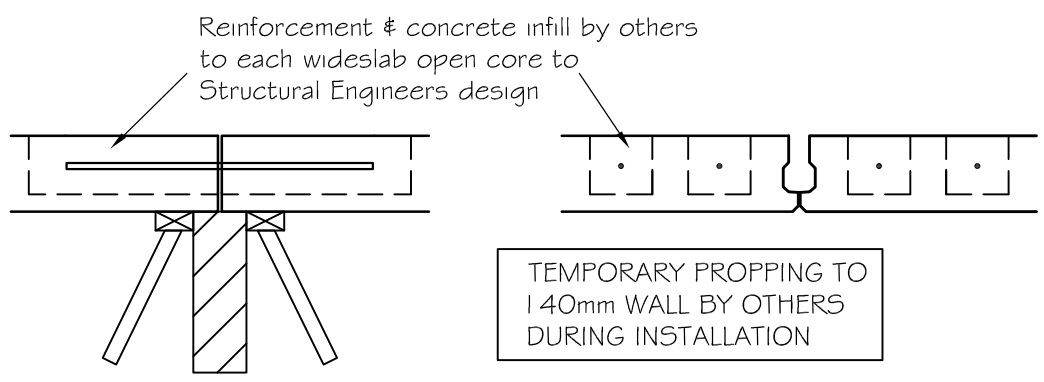
140mm SHARED BEARING WALL DETAIL
