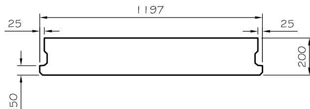
200mm DEEP WIDESLAB DIMENSIONS
