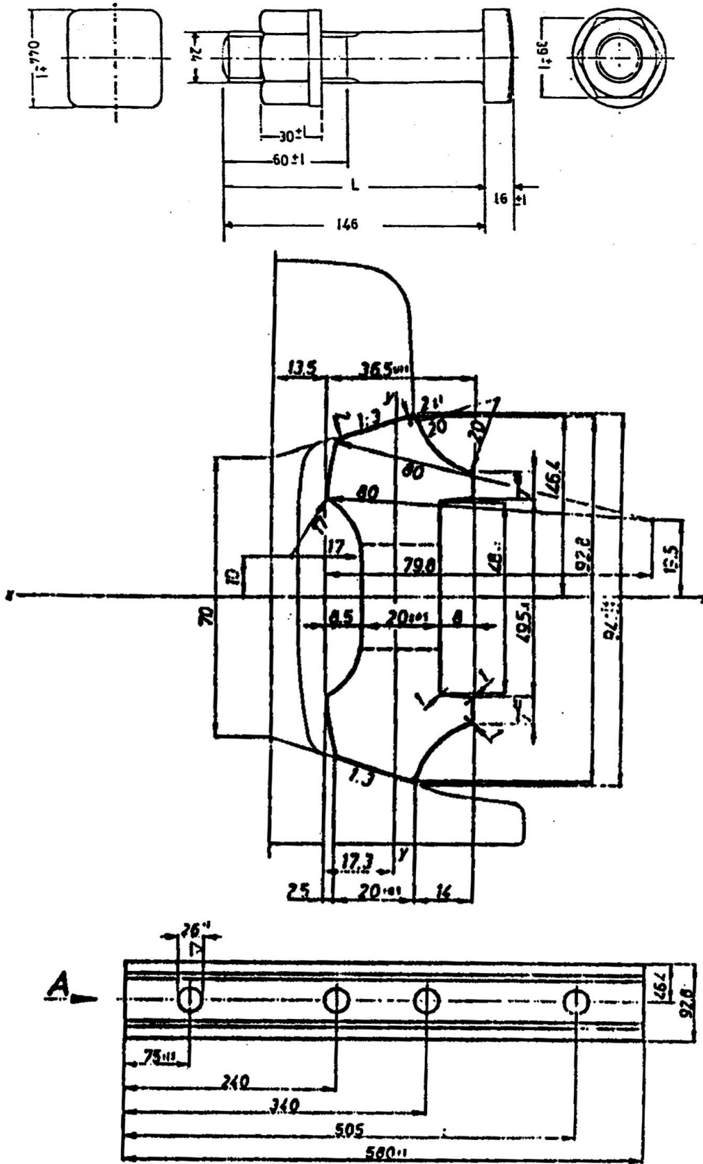
FISH PLATE S.49
