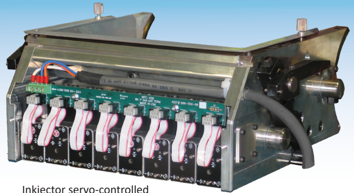
Inkjector servo-controlled keys on an ink fountain
