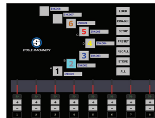
Main and secondary Inkjector control screens that display on the decorator's HMI
