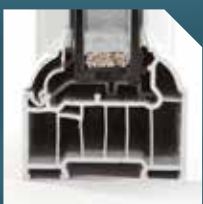
6-chamber profile
