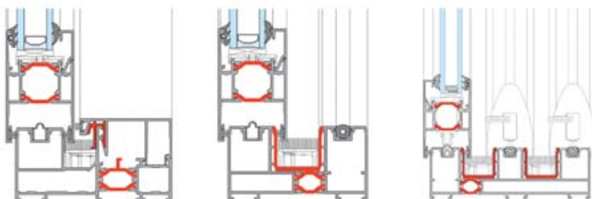
Single Track
