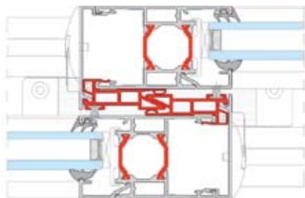
Interlock Detail
