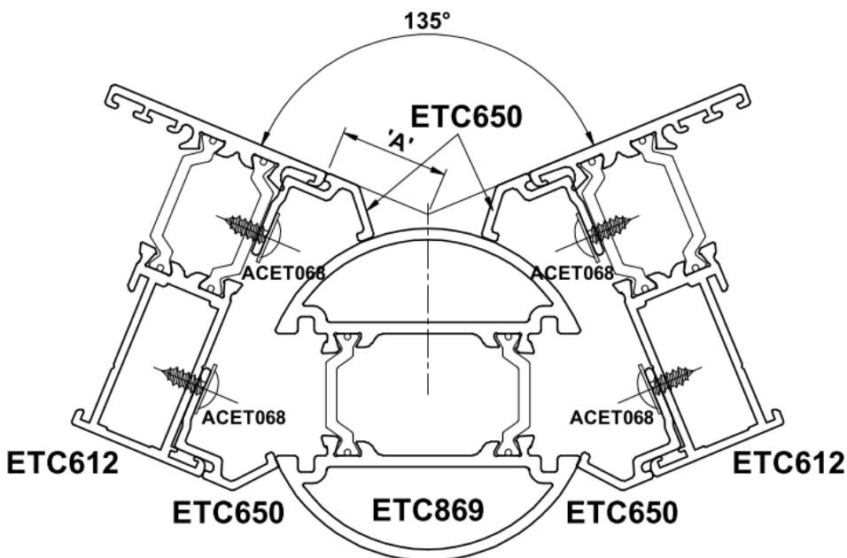
ETC869 Bay Pole with ETC650 frame adaptors for ETC612 59.5mm frame
