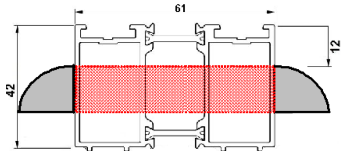
ETC656N 61mm x 42mm Extension for ETC610 & ETC612 (Small lip is noticeable to the front as this extension is 1.5mm wider than the outerframe)
