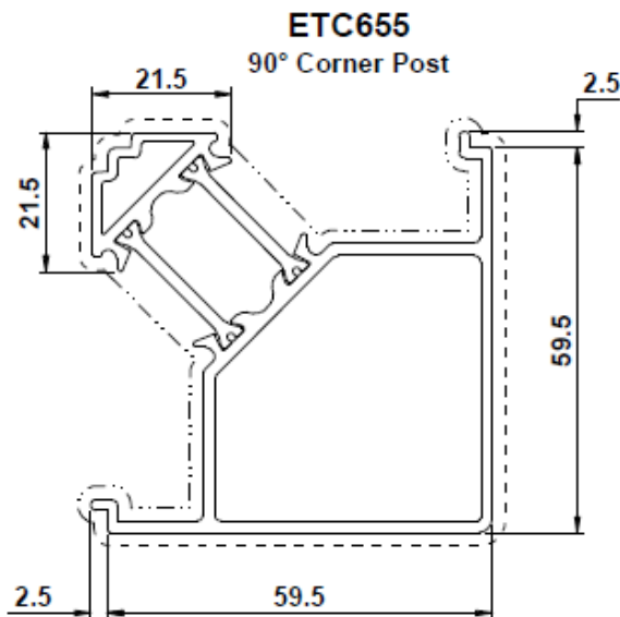
90° Corner Post ETC655 for ETC610 & ETC612
