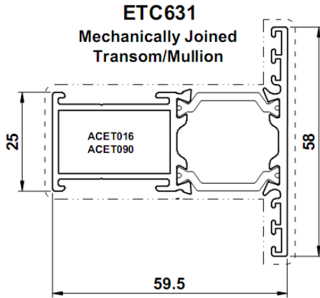
Standard Transom/Mullion (Ovolo tran/mull not available)
