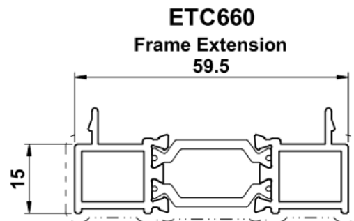
ETC660 59.5mm x 15mm Extension for ETC610 & ETC612
