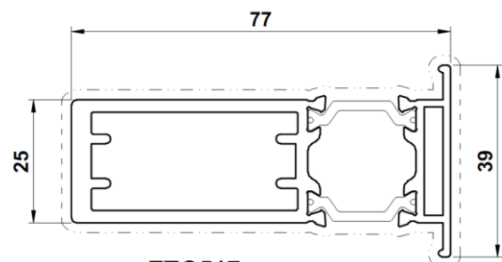
ETC517 Coupler
