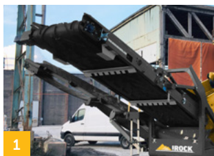
1 Discharging oversized material at 11' 1" (3.38m), the 42" (1050mm) wide 3-ply belt allows for efficient stockpiling.
