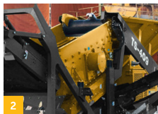
2 4' x 9' high energy screenbox delivers the most aggressive screening action in its class.
