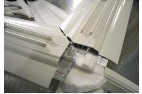
Fit the ridge top caps to the ridge body as per the photo above. Note the removal of the creasting upstands.
