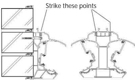
Make sure the correct position is struck when fitting the top caps. In colder weather conditions a block of timber can be used to spread the impact over the PVC-U top cap.
