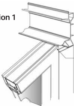
The wallplate sits on a corner post fitted between the house wall and gable window frame.
