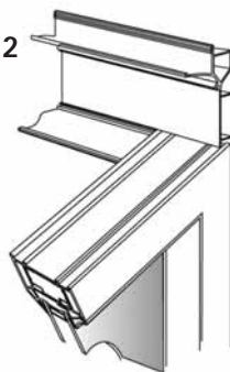
The wallplate is notched to fit around the gable window frame. This frame is fixed directly back to the house wall.
