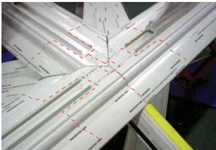
Fit the 3 separate ridge top caps leaving a tight mitred joint. Remove protective tape and apply lines of sealant as shown in red above. Note that the creasting track has been removed.
