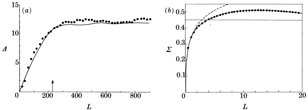
FIGURE 11. (a) Spectral rigidity \Delta(L) for rectangular billiard, continuing figure 4b to larger L . The circles were computed from the eigenvalues near the 20000th Casati et al. 1985); the smooth curve was obtained from the sum over closed orbits by Berry (1985); the arrow is the L corresponding to an energy range \hbar/T_{\min} , where T_{\min} is the period of the shortest closed orbit. (b) Number variance \Sigma(L) for 10^5 Riemann zeros near the 10^{12} th, continuing figure 8b to larger L ; the circles are plotted from data kindly supplied by A. M. Odlyzko; the smooth curve is the ‘semiclassical’ theory (adapted from Berry 1985), which predicts oscillation about the horizontal line \Sigma(\infty) = 0.4518 (= [\ln \ln (E/2\pi) + 1.2615]/\pi^2 , where (E/2\pi) \ln (E/2\pi e) = 10^{12} ); the dashed curve is for random complex matrices.
