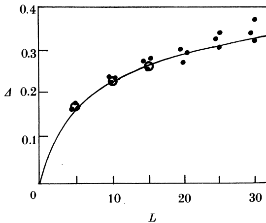
FIGURE 3. Spectral rigidity \Delta(L) for eigenvalues of the stadium billiard (filled circles, after Bohigas et al. 1984 a ) and the Sinai billiard (open circles, after Bohigas et al. 1984 b ), and the rigidity for random real symmetric matrices (smooth curve), whose asymptote is \Delta(L) \rightarrow (1/\pi^2) \ln L + \text{const.} as L \rightarrow \infty .
