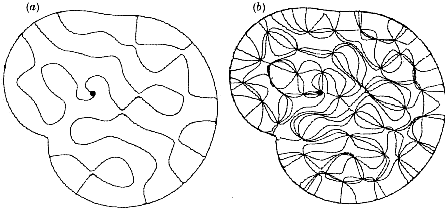
FIGURE 6. 50th eigenstate \psi of 'Africa' Aharonov-Bohm billiard with flux q\Phi/\hbar = \frac{1}{2}(\sqrt{5}-1) . (a) Nodal lines of \text{Re } \psi , which are very similar to the nodal lines of \psi with zero flux; (b) wavefronts (contours of phase of \psi ) at intervals of \frac{1}{4}\pi .
