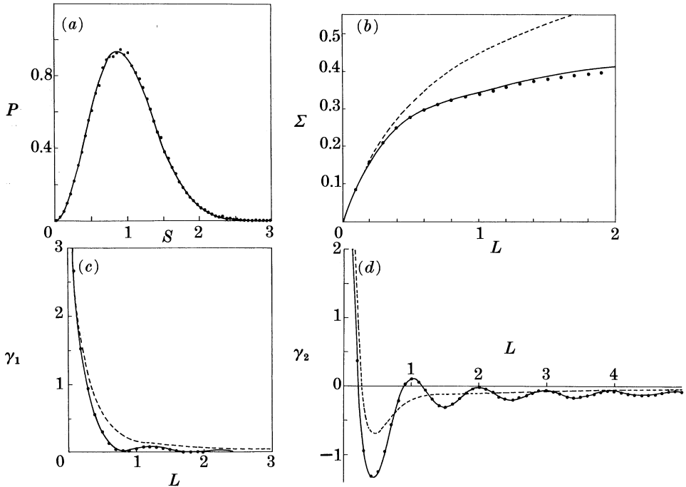
FIGURE 8. Statistics of imaginary parts of Riemann zeros, computed by A. M. Odlyzko. (a) P(S) (from Odlyzko 1987); (b) number variance \Sigma(L) \equiv \langle (n-L)^2 \rangle , where n is the actual number of zeros in an interval where the average number is L (the interval is 2\pi L/\ln(E/2\pi e) ) (from data kindly supplied by A. M. Odlyzko); (c) Skewness \gamma_1(L) \equiv \langle (n-L)^3 \rangle / \langle (n-L)^2 \rangle^{3/2} (kindly supplied by O. Bohigas); (d) excess \gamma_2(L) \equiv \langle (n-L)^4 \rangle / \langle (n-L)^2 \rangle^2 - 3 (kindly supplied by O. Bohigas). Full curves, random complex hermitian matrices; dashed curves, random real symmetric matrices.
