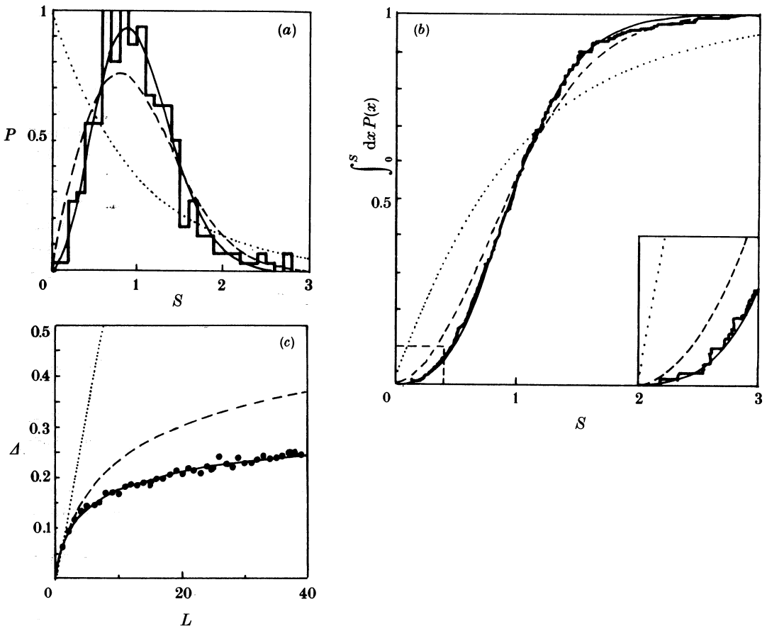
FIGURE 5. Level spacings distribution P(S) (histogram in (a)), cumulative level spacings distribution \int_0^S dx P(x) (histogram in (b)), and spectral rigidity \Delta(L) (circles in (c)) for eigenvalues of the Aharonov–Bohm ‘Africa’ billiard with flux q\Phi/h = \frac{1}{2}(\sqrt{5}-1) . The full curves are the statistics for random complex hermitian matrices, for which P(S) \approx (32/\pi^2) \exp(-4S^2/\pi) and \Delta(L) \rightarrow (1/2\pi^2) \ln L + \text{const.} as L \rightarrow \infty . The dashed curves are the statistics for random real symmetric matrices and the dotted curves are Poisson statistics.
