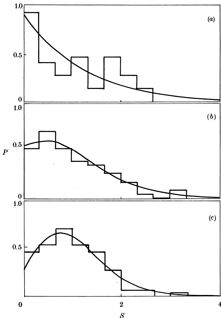
FIGURE 10. Level spacings distributions P(S) for even-parity, zero-angular momentum energy levels of a hydrogen atom in a 6T uniform magnetic field, for three different energy ranges with different phase-space fractions q of regular orbits: (a) -130 \text{ cm}^{-1} < E < -100 \text{ cm}^{-1} ( q = 0.71 , 47 levels); (b) -100 \text{ cm}^{-1} < E < -70 \text{ cm}^{-1} ( q = 0.32 , 71 levels); (c) -70 \text{ cm}^{-1} < E < -40 \text{ cm}^{-1} ( q = 0.16 , 116 levels); the smooth curves are P(S) for superpositions of Poisson and random real symmetric matrix spectra. (From Wunner et al. 1986.)
