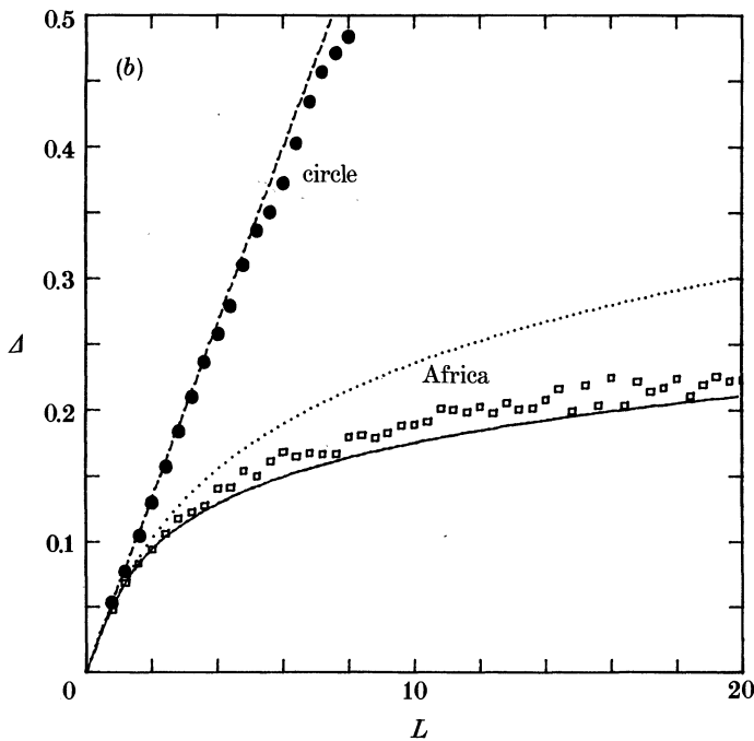
FIGURE 9. (a) Cumulative level spacings distribution \int_0^S dx P(x) and (b) spectral rigidity \Delta(L) , for neutrino 'Africa' and neutrino circle billiards. Full curves, random complex hermitian matrices; dotted curves, random real symmetric matrices; dashed and chain curves, Poisson statistics.
