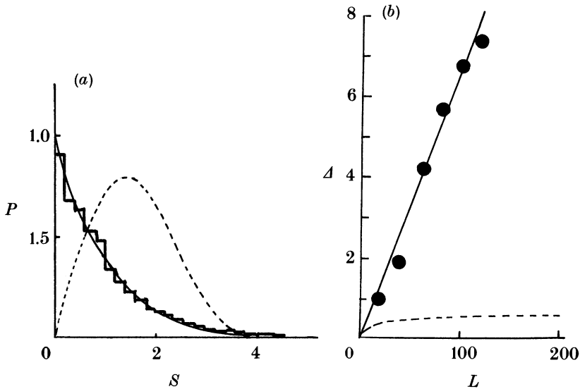
FIGURE 4. Level spacings distribution P(S) (histogram in (a) and spectral rigidity \Delta(L) (circles in (b)) for eigenvalues of the rectangular billiard. The full curves are the statistics for Poisson-distributed eigenvalues ( P(S) = \exp(-S) and \Delta(L) = \frac{1}{15}L ) and the dashed curves are the statistics for random real symmetric matrices.
