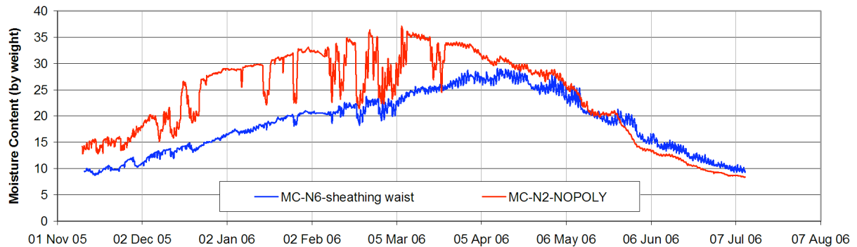
Figure 2.13: Moisture content of Sheathing Wall N6 (open cell) versus datum wall without poly
