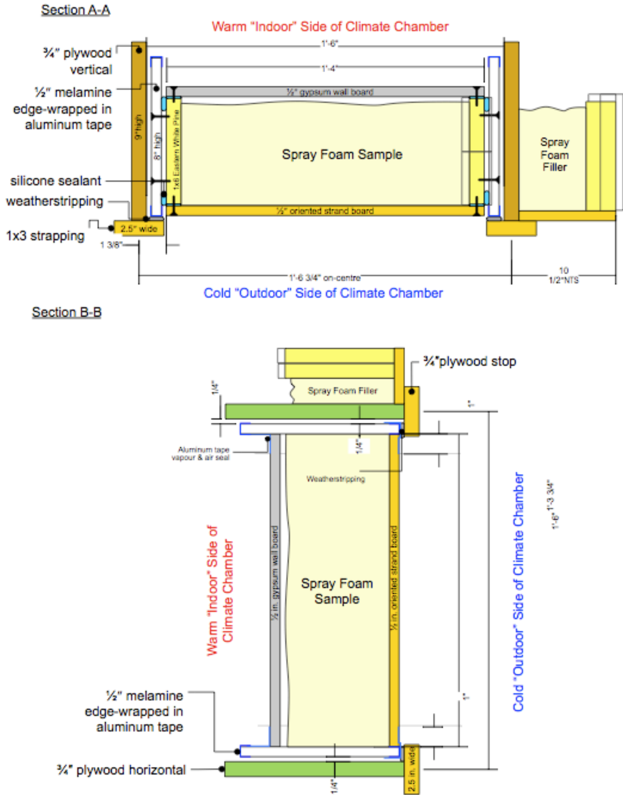
Figure 3.3: Sections Through Test Boxes
