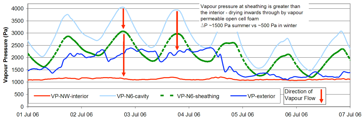
Figure 2.16: Wall N6 – Vapour Pressure Gradient during a typical summer week (July 1-7, 2006)
