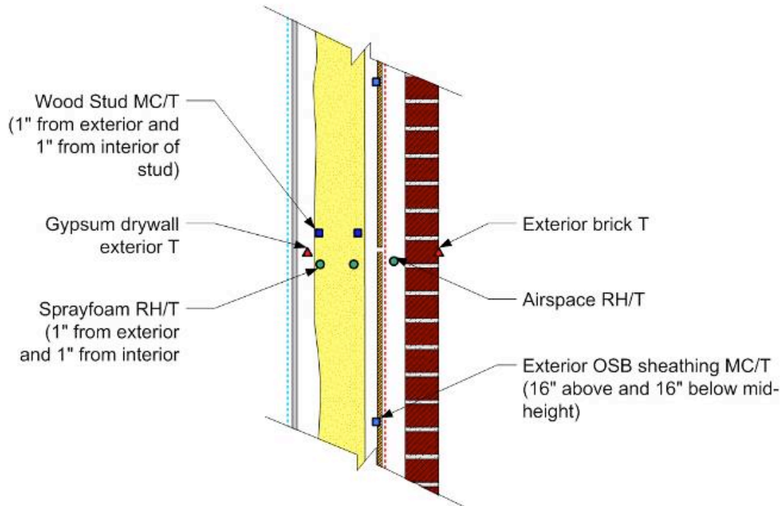
Figure 2.8: Wood Stud Wall Assembly (Walls 6, 7, 8) close-up of sensors
