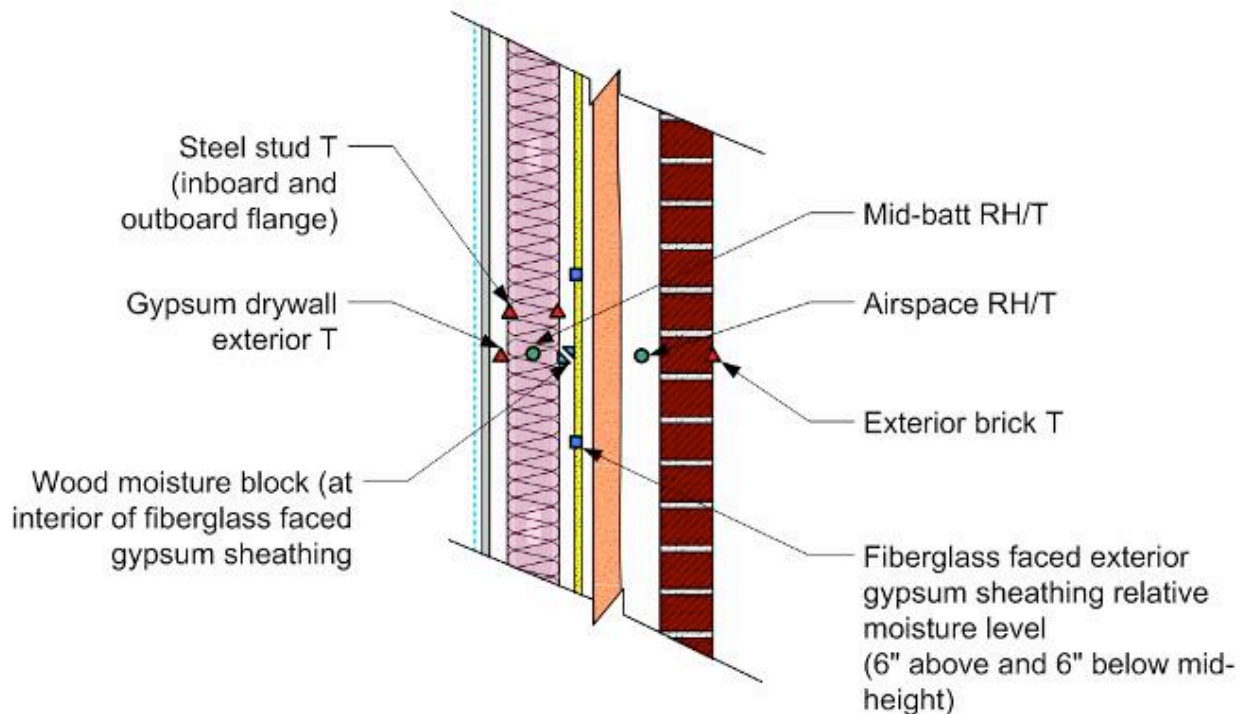
Figure 2.9: Steel Stud Wall Assembly (Wall 9) close-up of sensors
