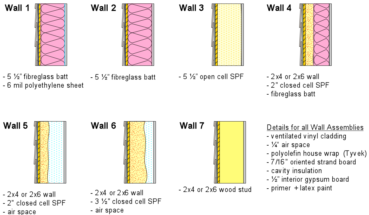
Figure 4.1: Cross-Sections of Wall Types Modelled
