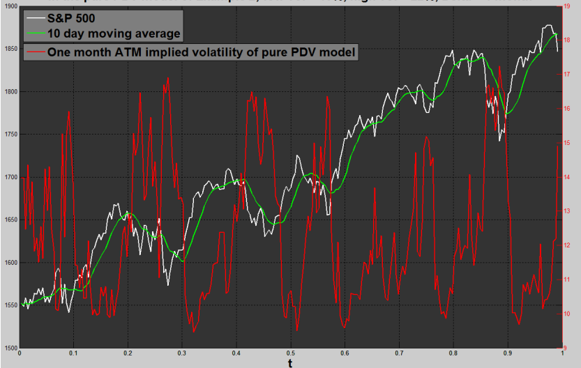
S&P500 from March 18, 2013 to March 18, 2014 and corresponding path of the 1M ATM implied vol in the pure PDV model of Example 2; low vol = 10%, high vol = 22%, Delta = 1 month
