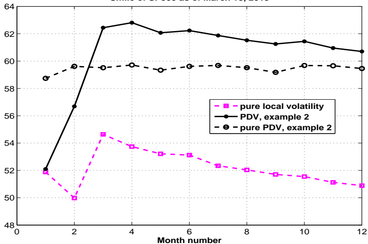
Price in % of forward starting one month digital ATM call Example 2: low vol = 10%, high vol = 22%, Delta = 1 month Smile of SP500 as of March 18, 2013
