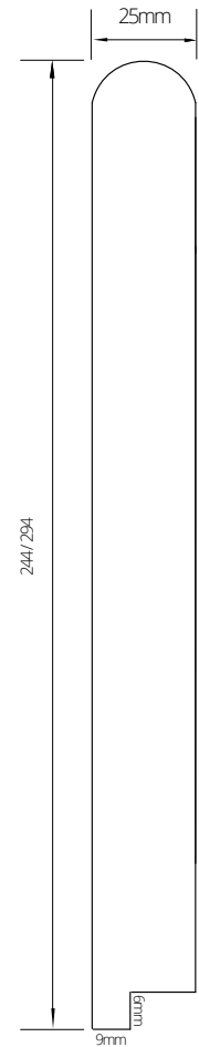
WINDOW BOARD 244/294 x 25 x 3660mm
