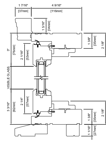
WOOD CASEMENT 4 9/16" (116mm)
