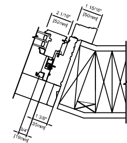
FRAMED WALL WOOD CASEMENT 6 9/16" (166 mm) JAMB
