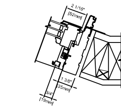
FRAMED WALL METAL CLAD CASEMENT 4 9/16" (116 mm) JAMB
