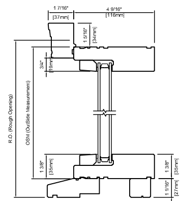
WOOD PICTURE 4 9/16" (116mm)
