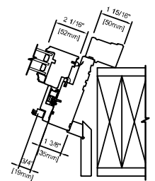
STRAIGHT WALL WOOD CASEMENT 6 9/16" (166 mm) JAMB
