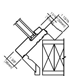
45° WOOD PICTURE 4 9/16" (116mm)
