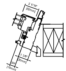
STRAIGHT WALL METAL CLAD CASEMENT 4 9/16" (116 mm) JAMB
