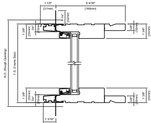
METAL CLAD PICTURE 6 9/16" (166mm)
