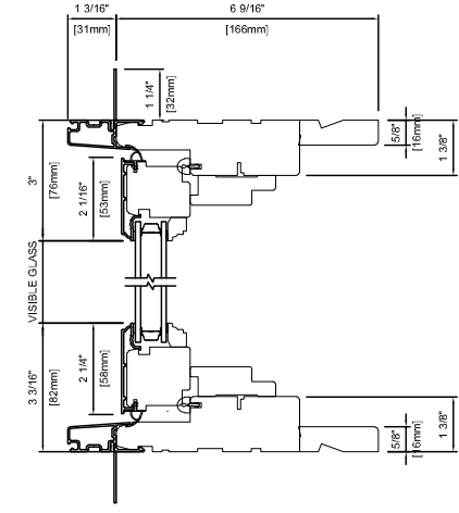
METAL CLAD CASEMENT 6 9/16" (166mm)
