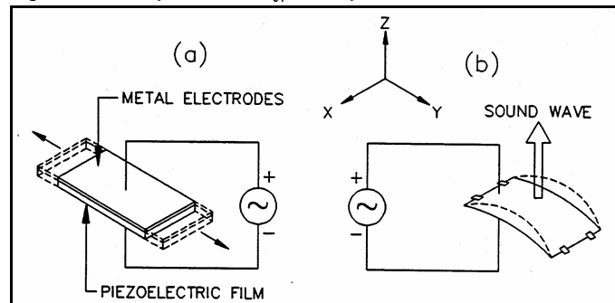
Figure 10. Clamped film in d_{31} mode produces sound
