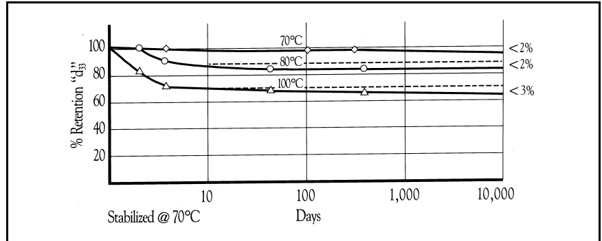
Figure 23. Thermal stability of d_{33} constant - 70^\circ\text{C} annealed PVDF
