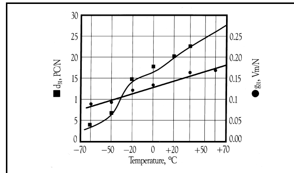
Figure 24. Temperature coefficient for d_{33} and g_{31} constants - PVDF
