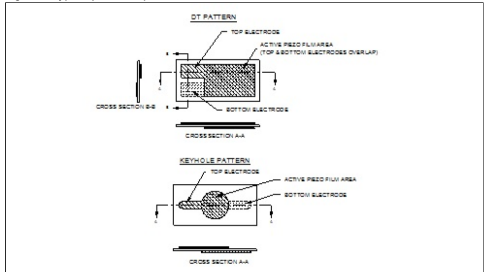
Figure 3. Typical piezo film patterns
