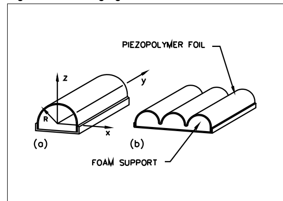
Figure 59. Air ranging ultrasound transducers
