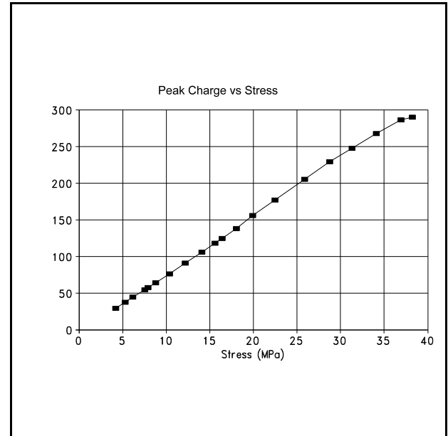
Figure 27b. Piezo cable linearity
