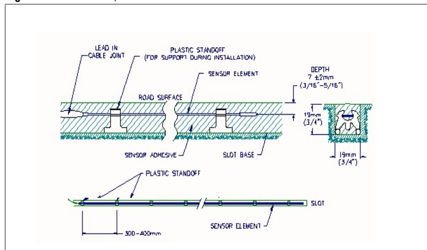
Figure 54. Permanent, In-The-Road Traffic Sensor
