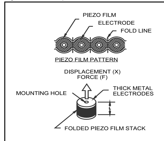
Figure 32. Folded piezo film actuator
