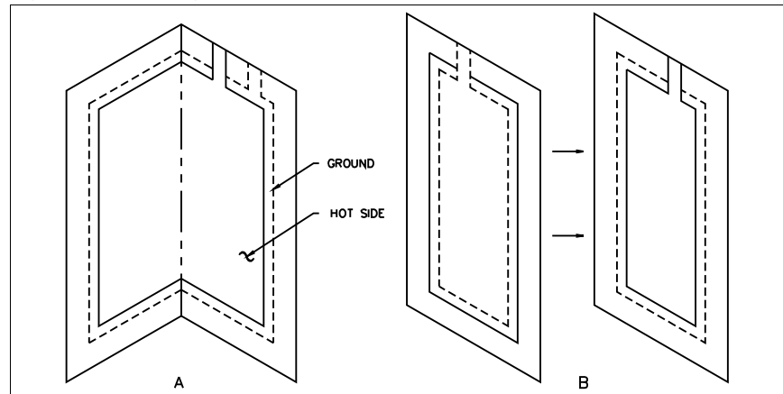
Figure 55. Shielding piezo film
