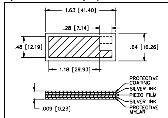
Figure 2. DT1 Element in [mm]
