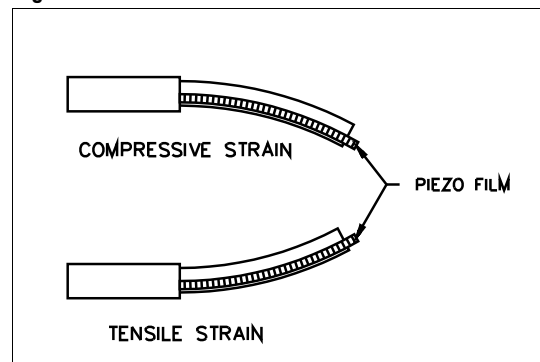
Figure 52. Beam switch
