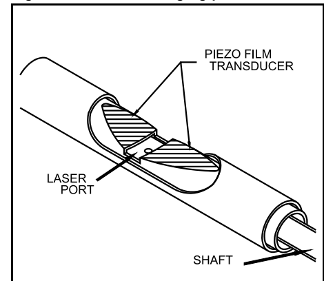
Figure 58. Invasive imaging probe
