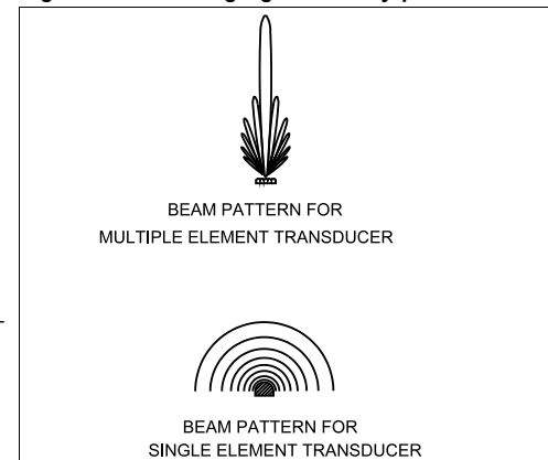
Figure 60. Air-ranging directivity patterns
