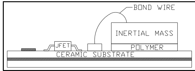
Figure 56. ACH-01-XX internal view
