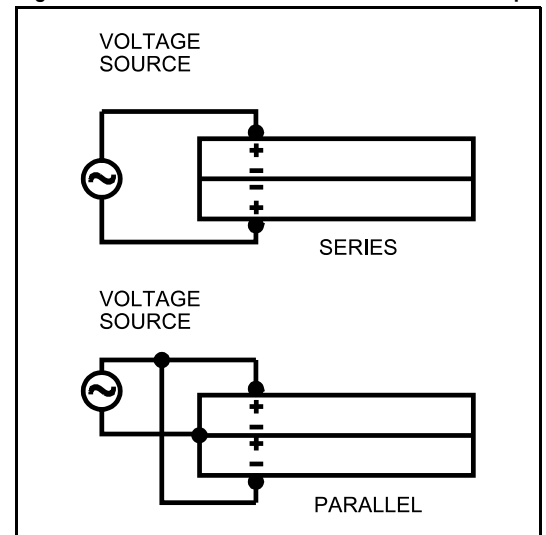
Figure 30. Lead attachment methods for a bimorph
