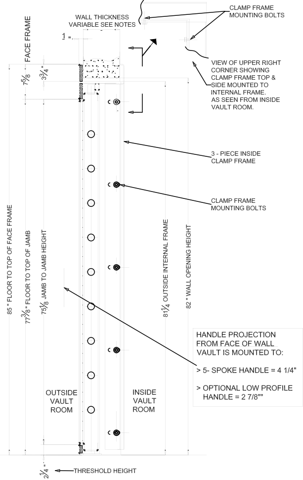
SECTIONAL SIDE VIEW OF FRAME
