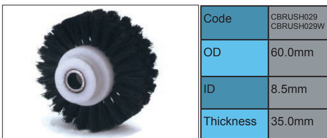
KBA / PLANETA - BRUSH029 - BROWN CARD KBA / PLANETA - BRUSH029W - WHITE PAPER NATURAL FIBRE
