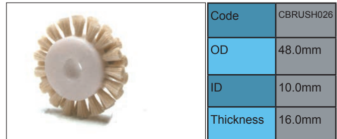
KBA 142 / 162 FOR CARD NATURAL FIBRE
