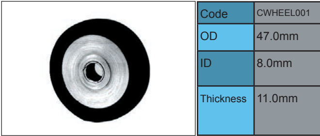
HEIDELBERG SORM /SORD / SORS / SM52-72-74-102 SOFT RUBBER WHEEL
