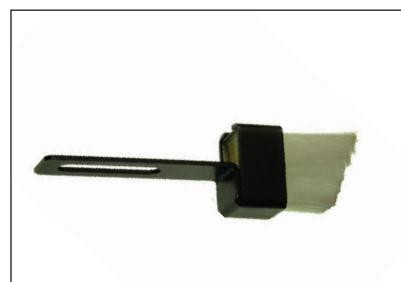
ROLAND / MAN SHEET STEADIER
