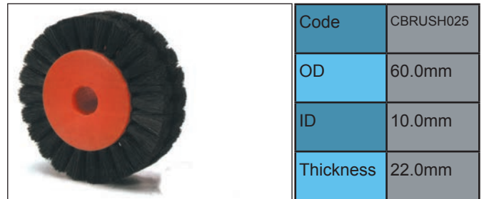
KBA 104 / 105 FOR CARD NATURAL FIBRE
