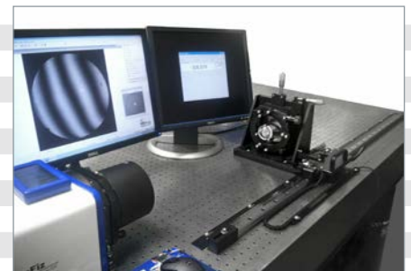
Digital Radius Slide for ROC Measurement
