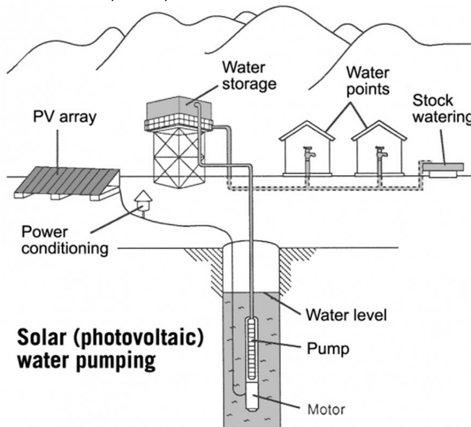
Figure 2: Solar (PV) water pumping system ( http://www.zimsolar.co.uk/LI_rural_solar_systems.html )
