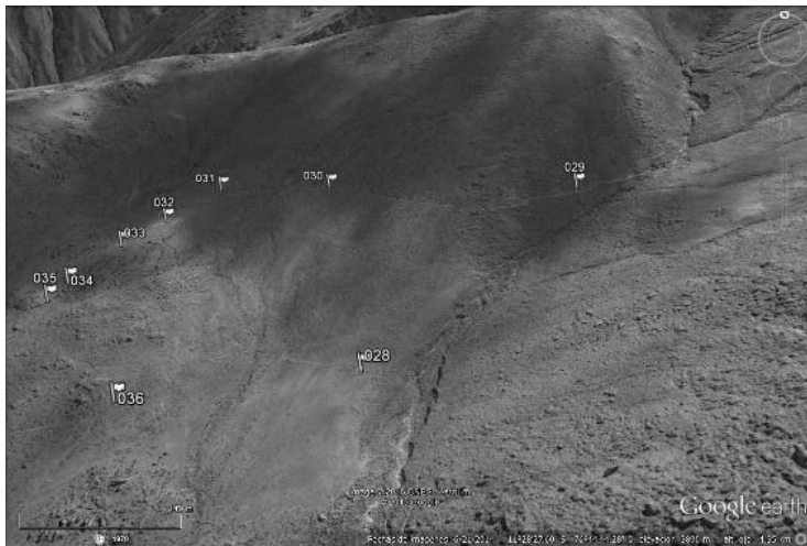
Fig. 7 - Rain runoff diversion canals start near points #28 and #29 from Pachipugro stream
