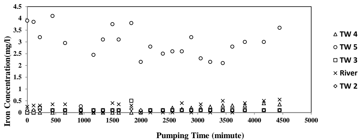
Figure (2.4): Iron variation during the testing.
