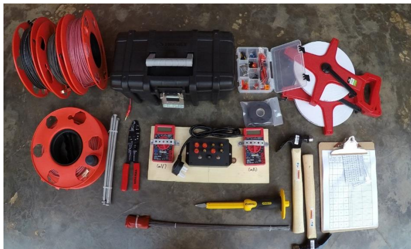
Figure 4: The Water4 resistivity toolkit consisting of control box, wire cable, spike electrodes, multimeters, measuring tapes, inverter and repair supplies.
