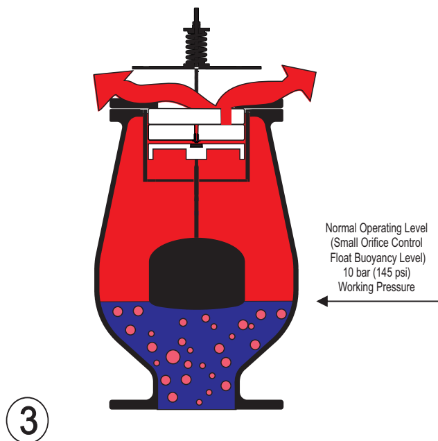
3 PRESSURIZED AIR/GAS RELEASE PIPELINE OPERATING
