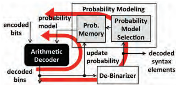
Figure 2: Feedback loops in CABAC entropy decoding engine.
