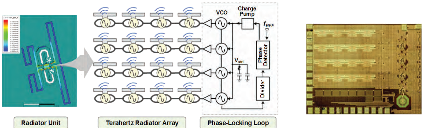
Figure 1. A terahertz radiator array with integrated phase-locking loop. Each unit inside the array enables maximum oscillation, optimum harmonic generation, as well as efficient on-chip radiation [R. Han, et al, ISSCC 2015].
