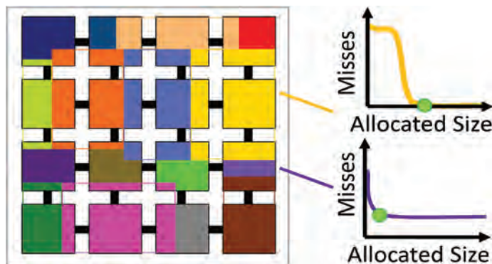
Figure 3: Jigsaw gangs physically distributed cache banks into virtual caches, which are sized to minimize cache misses and placed close to the threads that use them.
