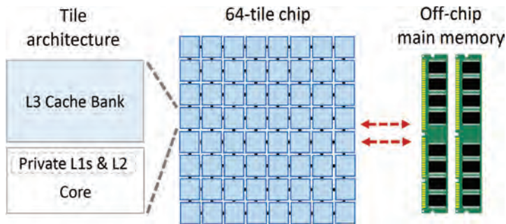
Figure 2: A tiled 64-core chip with a distributed cache hierarchy.
