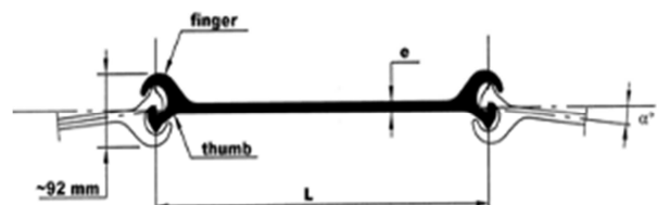
Figure 7 Exemple de palplanche plate. Source: ArcelorMittal
