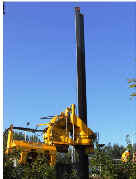
Figure 34 Exemples de vérineurs silent piler giken ECO 700S. Source : GIKEN.co.uk
