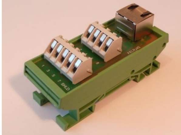
FELRJ45
