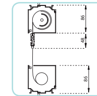
C85/C185 cassette
