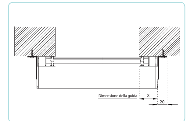
Front fix
