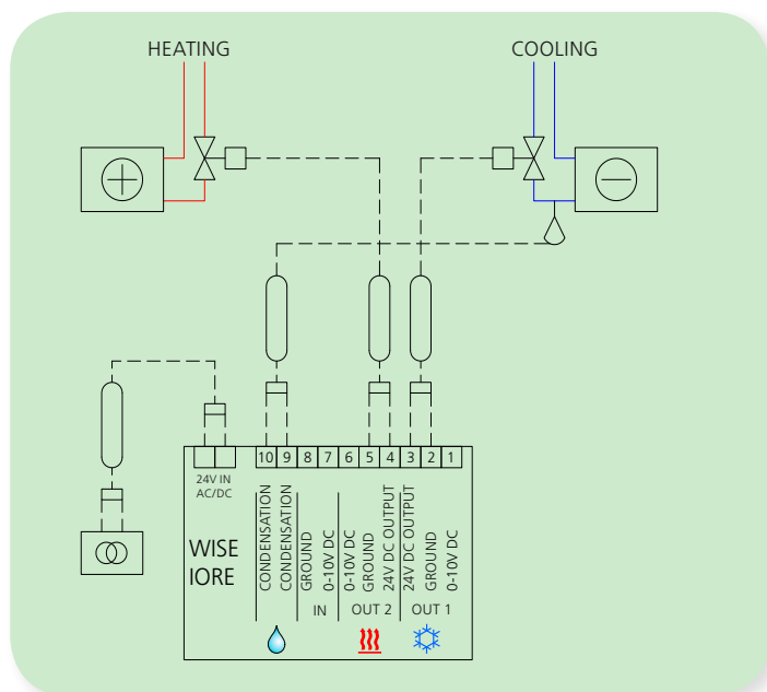
IORE controlling heating and cooling thermo-actuator and condensation sensor
