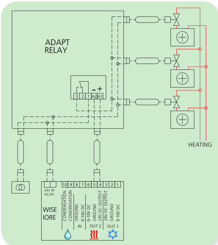
IORE controlling radiator heating 3 or more thermo-actuators
