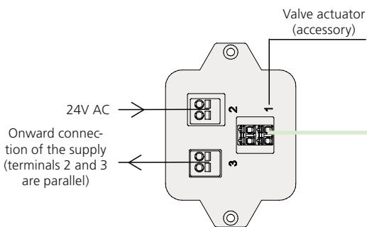
WISE Sphere C, diffuser connection
