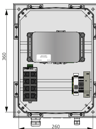
Holes for installation, SuperWISE II, SuperWISE II SC. 4x installation screws (clearance hole \varnothing = 8 mm), screw selection based on the substrate.
