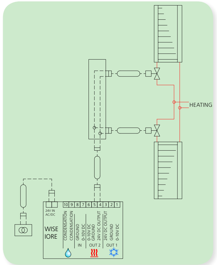
IORE controlling radiator heating 2 thermo-actuators
