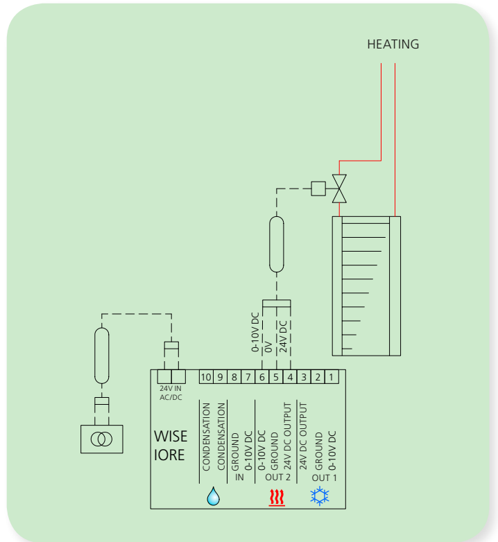
IORE controlling radiator heating 0-10 V
