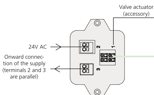
WISE Colibri C, diffuser connection
