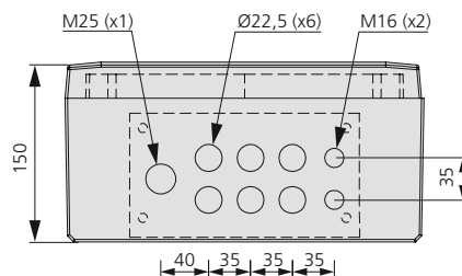
SuperWISE II, SuperWISE II SC, underside.
