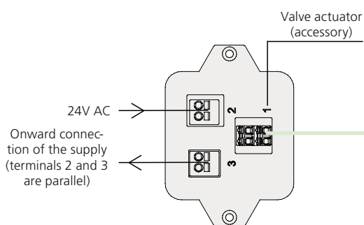
WISE Sphere F, diffuser connection
