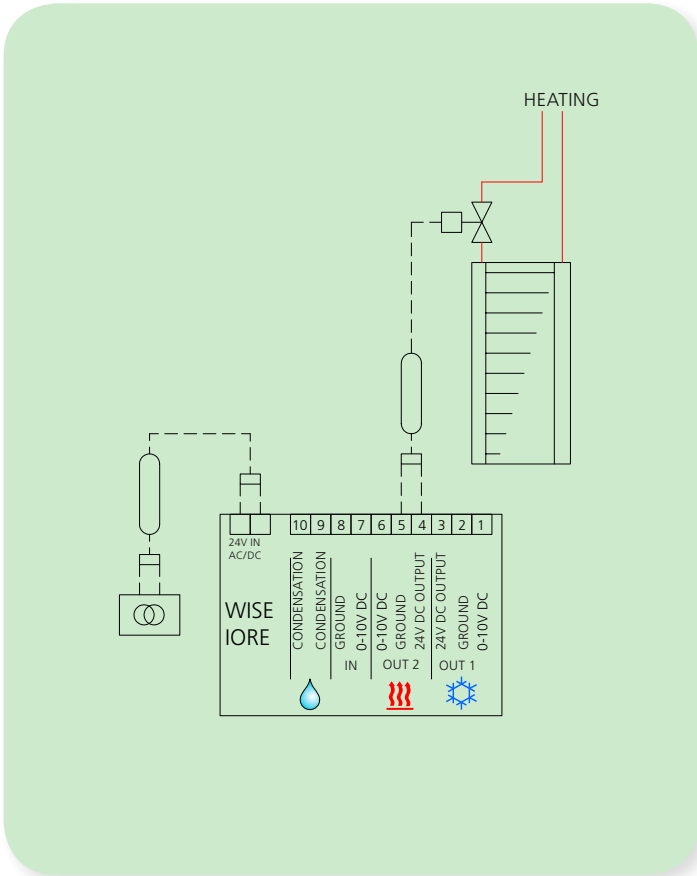
IORE controlling radiator heating 1 thermo-actuator
