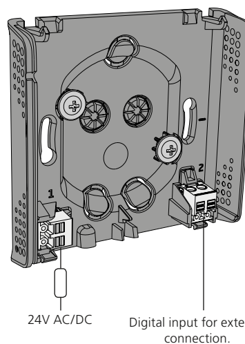
WISE RTA - back-piece, power supply and connection
