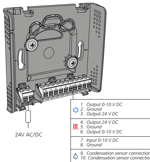
WISE IORE - back-piece, power supply and connection
