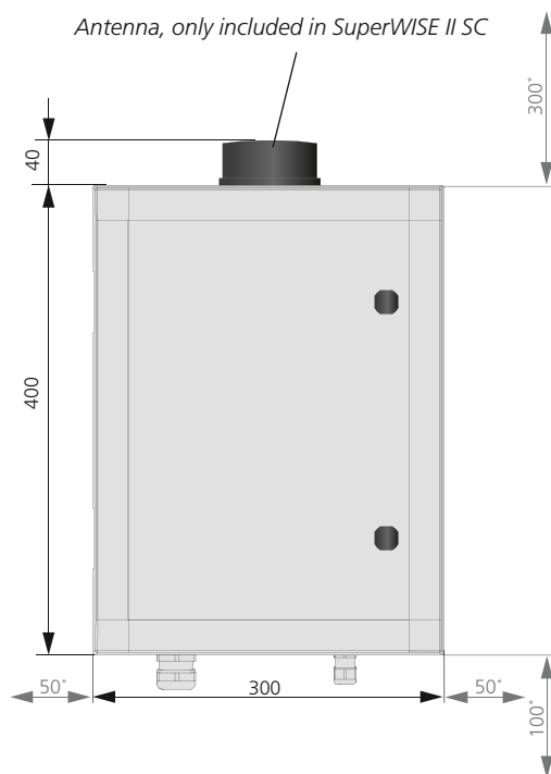
SuperWISE II, SuperWISE II SC, measurement figure. *Minimum free clearance to nearby installations.
