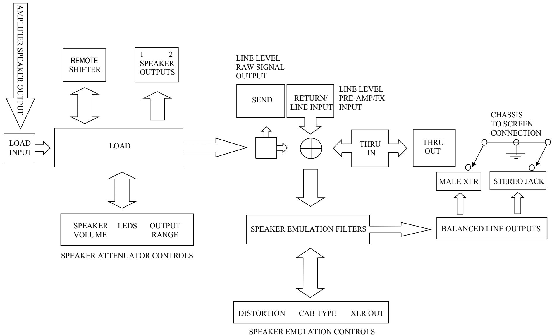
SEQUIS MOTHERLOAD ELEMENTAL BLOCK DIAGRAM
