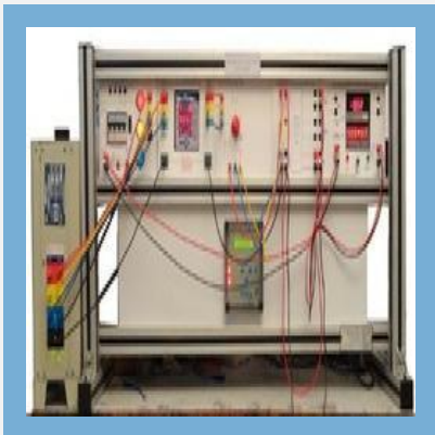
Under/Over Voltage Relay Trainer
