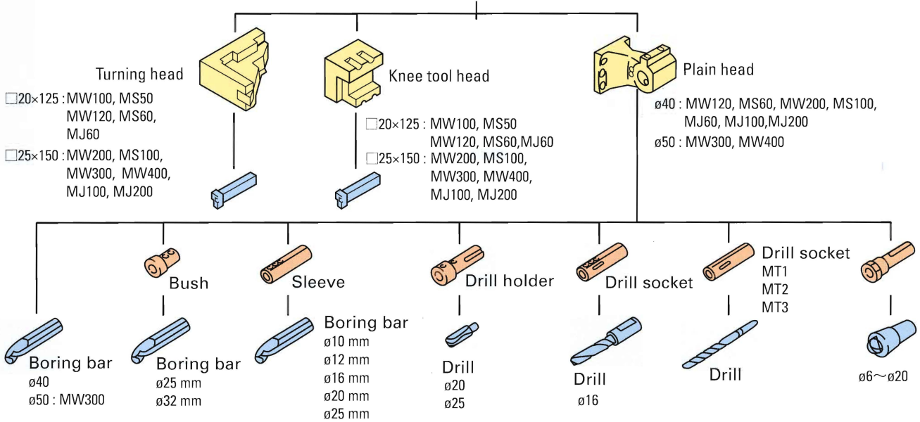
8 Station Turret : MW120, MS60, MW400, MJ60
