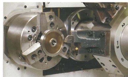
Turret Axis Track Back
