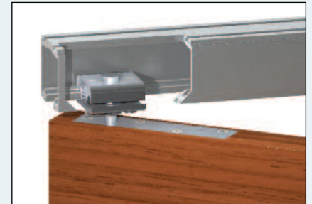
Top pivot assembly for F-50
