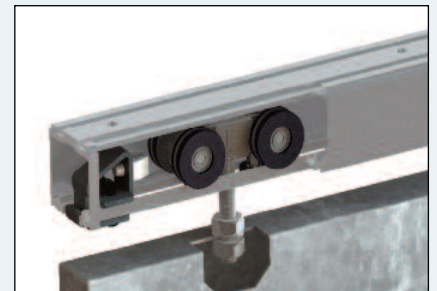
Soffit fixed 180 track c/w hanger for metal door
