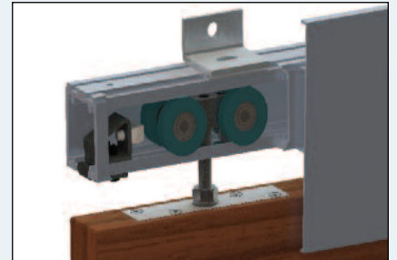
Wall fixed 250 track c/w fascia, hanger and apron plate for timber door
