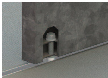
Recessed floor guide and channel for metal doors
