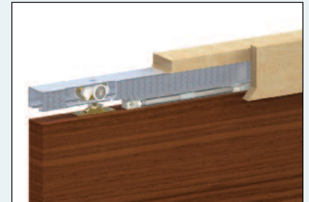
Track c/w hanger and integrated soft closer
