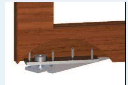
Bottom pivot assembly for F-50
