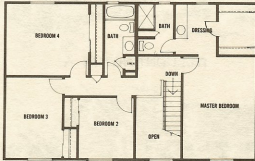
UPPER FLOOR
