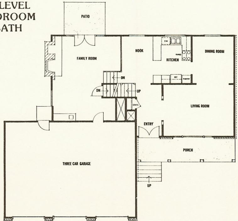
MAIN FLOOR
