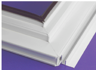
Engineered PVCu internal frame with secure welded corners
