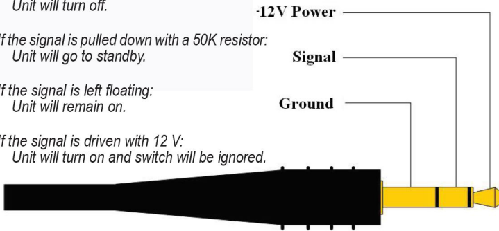
12 Volt Remote Trigger wiring.
