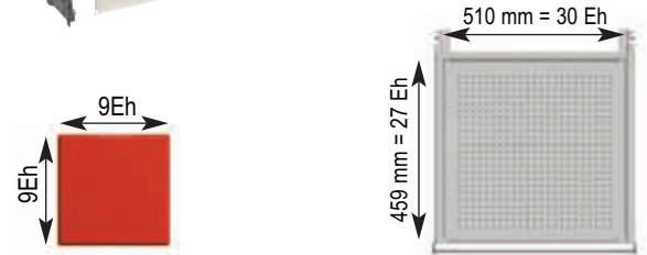
Drawers
