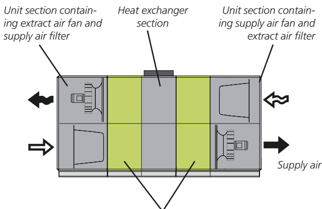
Up to two multisections can be used for one air handling unit. The illustration shows possible locations of the multisection.
