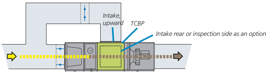
Solution for fire bypass (upwards, back or inspection side) for GOLD SD 004-012 extract air handling unit in split version.
