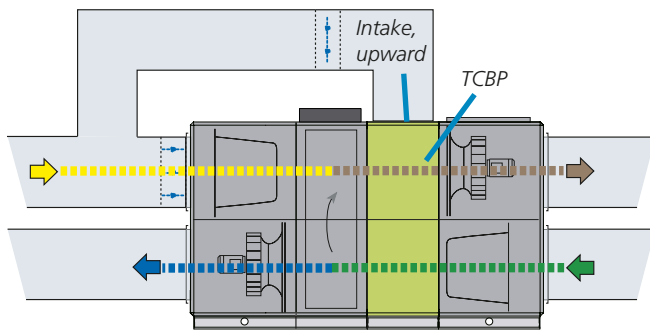
Solution for fire bypass (upward) for GOLD RX 004-080.
