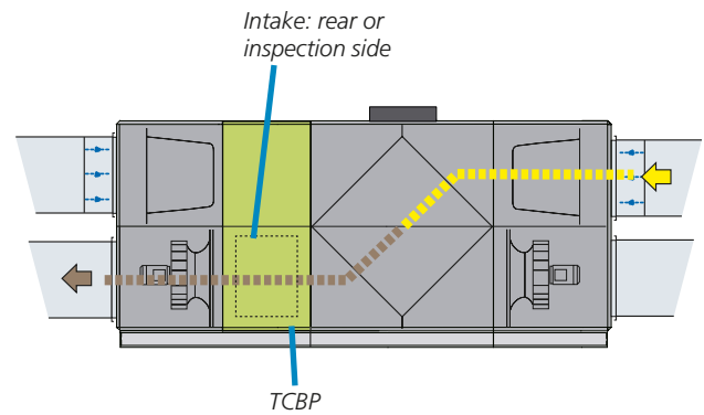
Solution for fire bypass (rear, inspection side or upward) for GOLD PX 004-040.
