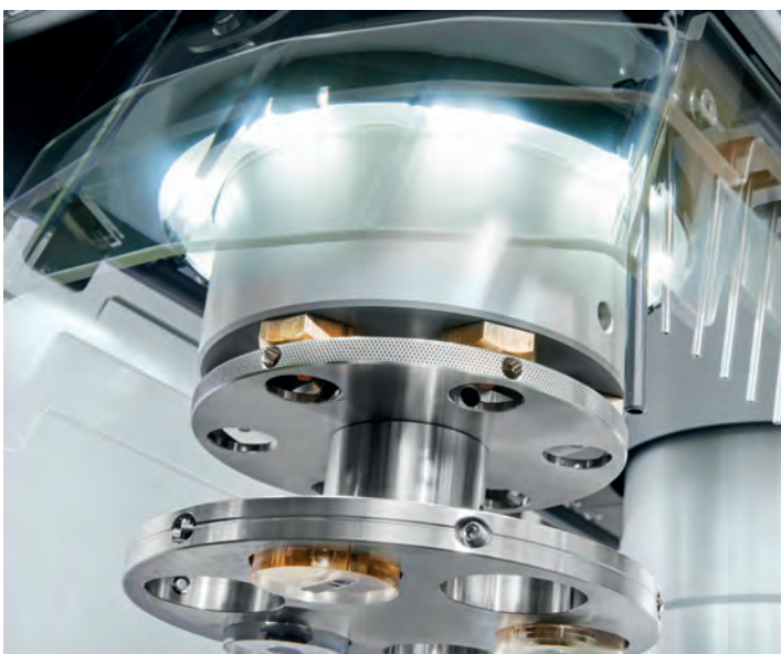
SAPHIR 550 Polishing head and diamond dispenser
