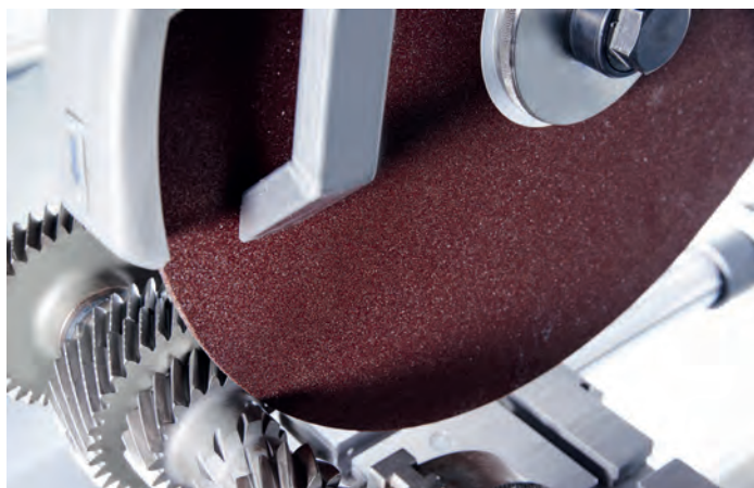
Abrasive sectioning
