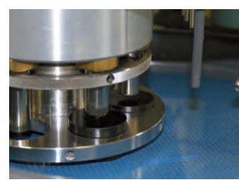
Individual Pressure Holder
