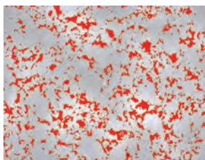
Coating porosity - Axio Imager 2
