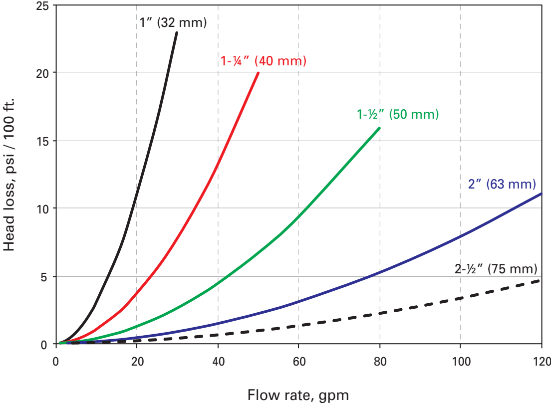
PRESSURE LOSS VS FLOW RATE 1" THRU 2-1/2", SDR 9
