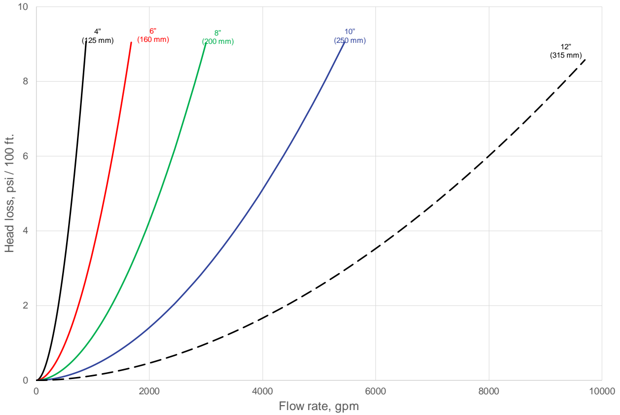
PRESSURE LOSS VS FLOW RATE 4" THRU 12", SDR 17.6
