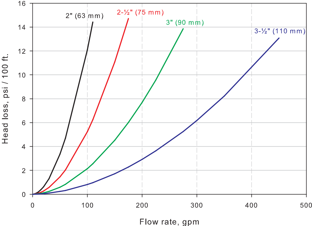
PRESSURE LOSS VS FLOW RATE 2" THRU 3-1/2", SDR 7.4
