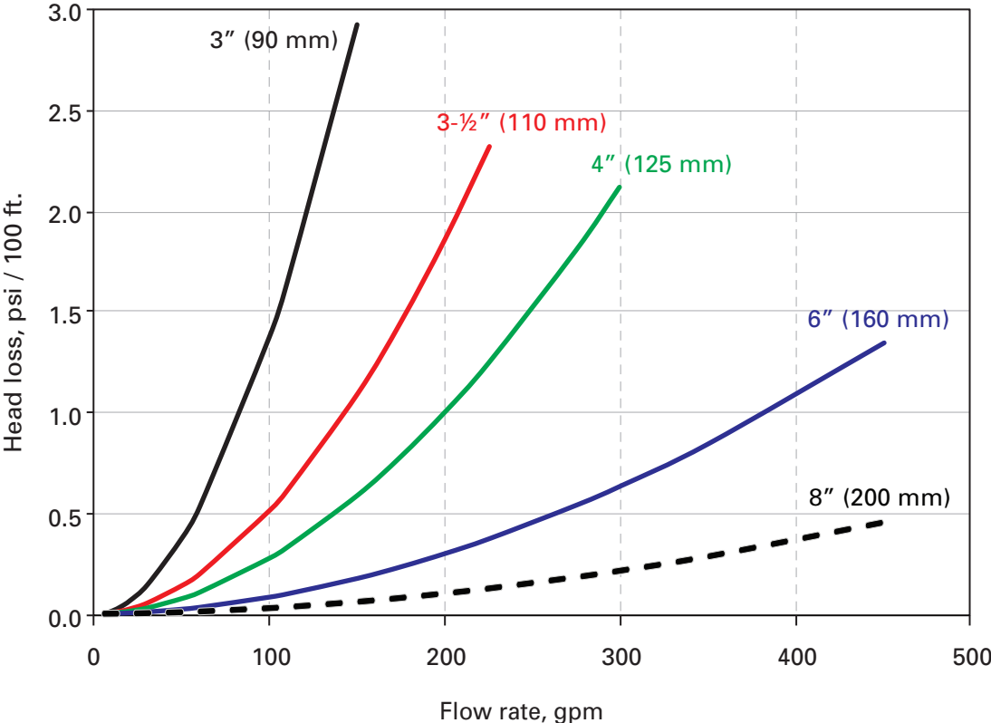
PRESSURE LOSS VS FLOW RATE 3" THRU 8", SDR 9
