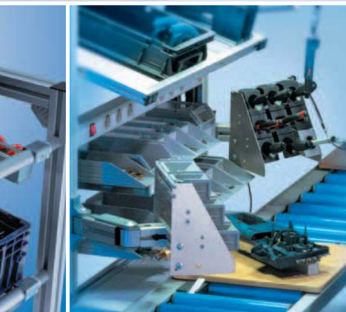
Multi-angle quick connector securely connects two profiles at any angle.
