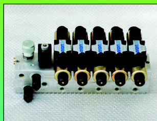
ELECTROHYDRAULIC DISTRIBUTOR WITH ELECTRIC CONTROLS
