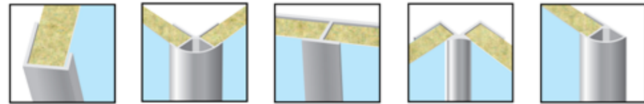
End Cap Silver 25013 White 25018 Black 69994 Polished 25028 External Corner Silver 25012 White 25017 Black 69993 Polished 25027 H Joint Silver 25014 White 25019 Black 69995 Polished 25029 Internal Corner Silver 25051 White 25016 Black 69992 Polished 25026 Quadrant End Cap Silver 25015 White 25020 Black 25025 Polished 25030
