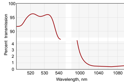
031-6500. HR > 99.5% @ 1064 nm, HT > 93% @ 532 nm, AOI = 0°
