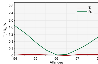
420-1258UHT. Ultra High Transmission @ 1064 nm, T_s < 0.2\% , R_p < 0.2\% , AOI=56°
