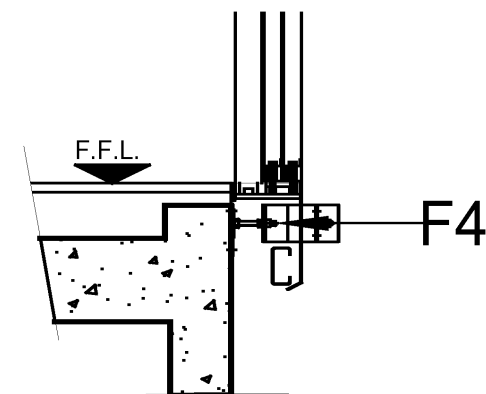
Lift Entrance Details Concrete Level
