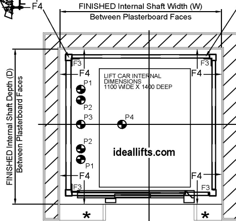
Ideal Lifts 8 Person 800 wide Two Panel Side Opening Doors Lift Plan
