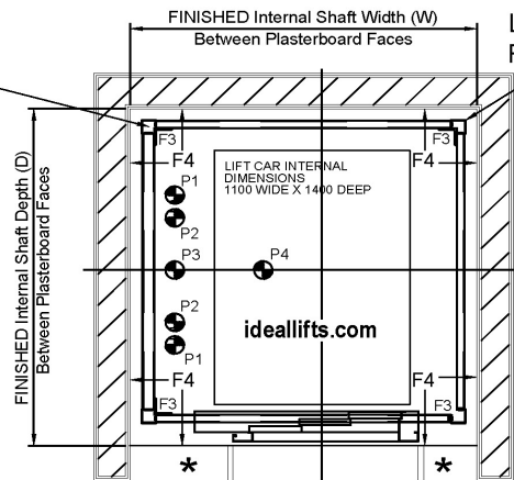
Ideal Lifts 8 Person 900 wide Three Panel Side Opening Doors Lift Plan
