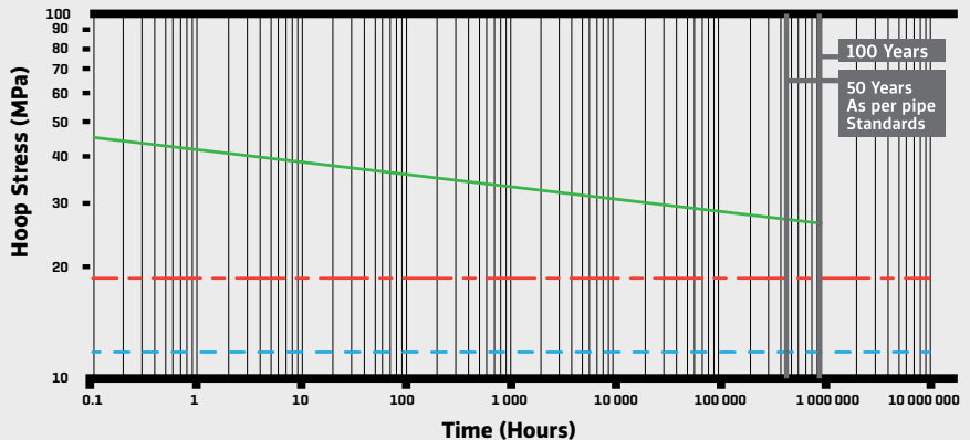
Stress-Time line for PVC-U and PVC-M at 20°C. [1]
